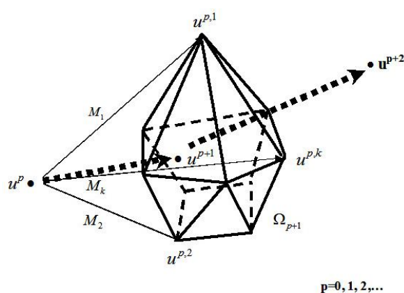
Fig. 1. Scheme of the multifunction method of searching of the extremum, founded on parallel using forming its methods M_1, M_2, \dots, M_k .
